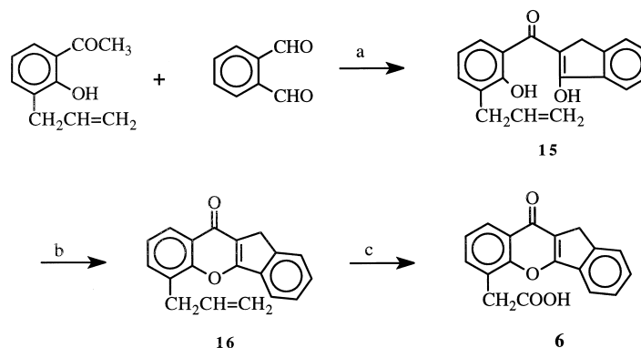
Scheme 2. Reagents: (a) KOH 50%, room temperature, 12 h; (b) HCl(g), MeOH reflux 2 h; (c) KMnO 4 , 0–5 °C, 6 h.
