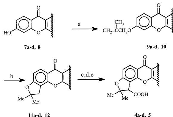
Scheme 1. Reagents and conditions: (a) methylallylbromide, K 2 CO 3 reflux; (b) 2,6-dimethylphenol 230–240 °C, 8 h; (c) NBS; (d) CuCN; (e) AcOH, H 2 SO 4 , H 2 O reflux, 2 h.
